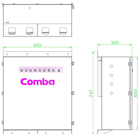
AC-DC Battery Unit
