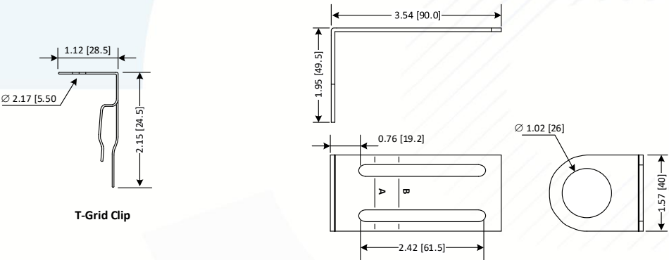
Aluminum Bracket
