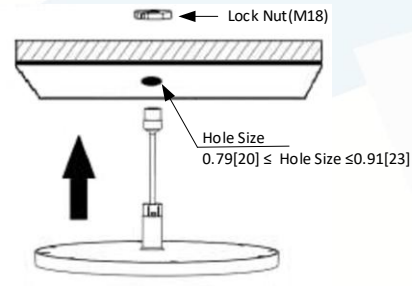
Fig 2. Making hole on the acoustic ceiling board
