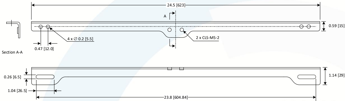
Aluminum Frame
